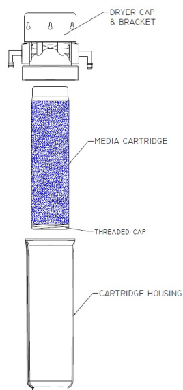
Figure 1. DI Dryer 2.0 Exploded View
