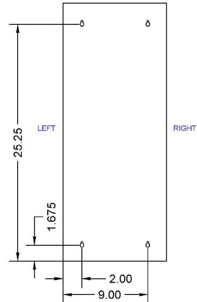
CHASSIS - BACK VIEW
