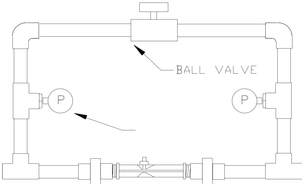
Figure One: Venturi Injector Bypass Assembly
