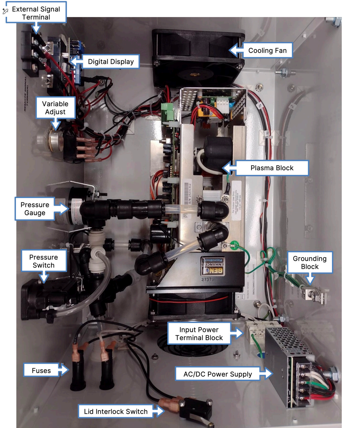
Figure 6: AIM P7 Internal Components
